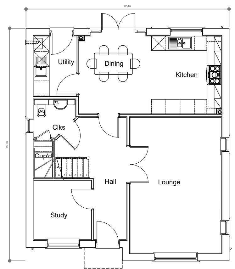
Ground Floor Plan Area = 139.12m 2 (1496 sq ft)
